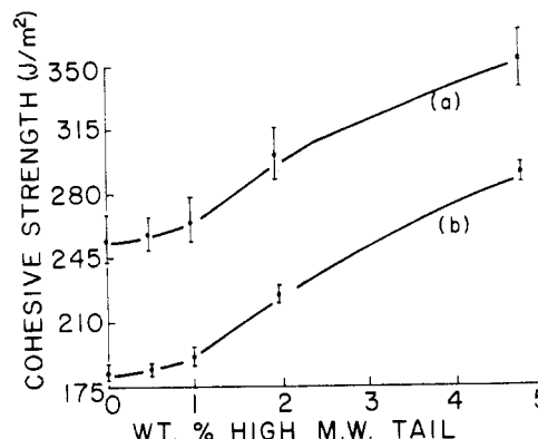
Figure 7. Cohesive strength (measured in a 180° peel geometry) of uncured PB elastomer of M_w = 115000 ( PI = 1600 ), measured as a function of the added concentration of PB of M_w = 702000 . Nominal strain rate and test temperature, respectively, were (a) 33 s -1 and 23 °C, (b) 3.3 s -1 and 0 °C.
